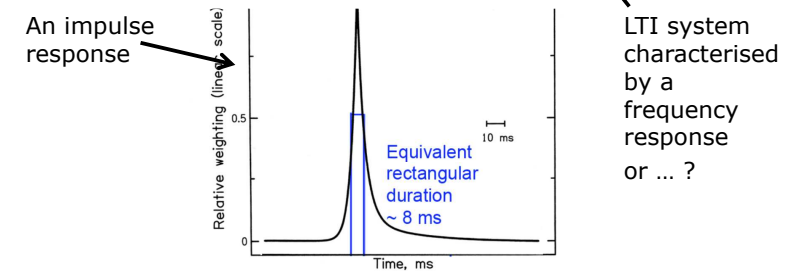
FIGURE 5.10 The "shape" of the sliding temporal integrator (window). This is a weighting function applied to the output of the nonlinear device. It performs a weighted running average of the output of the nonlinear device. The shape is plotted on a linear scale as a function of time.
